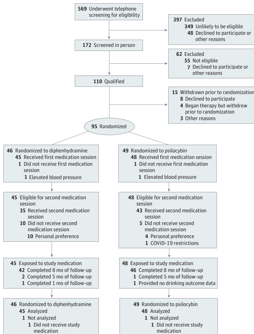
Figure 1. CONSORT Diagram
